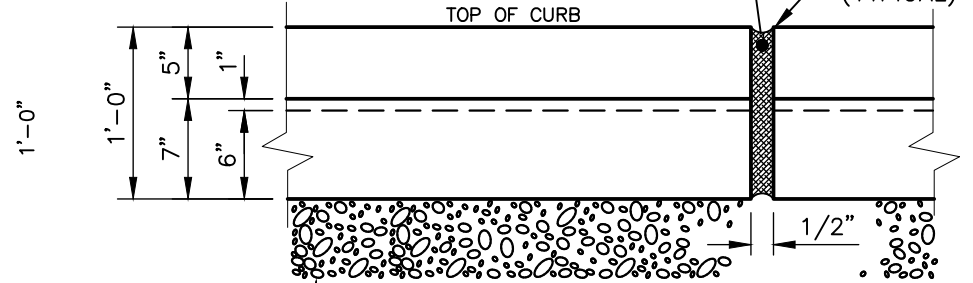
FRONT VIEW TRANSVERSE EXPANSION JOINT
