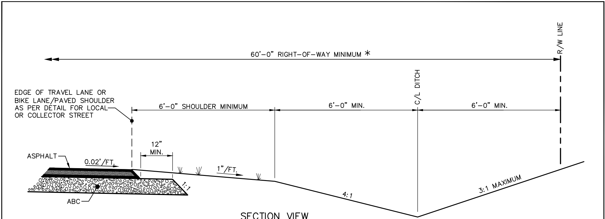
SECTION VIEW
