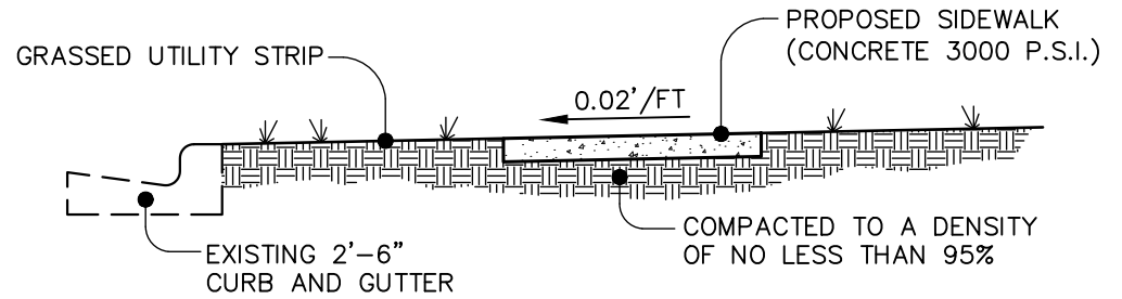
TYPICAL SECTION
