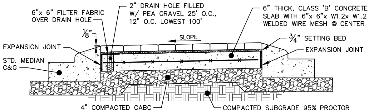
BRICK PAVER MEDIAN SECTION VIEW
