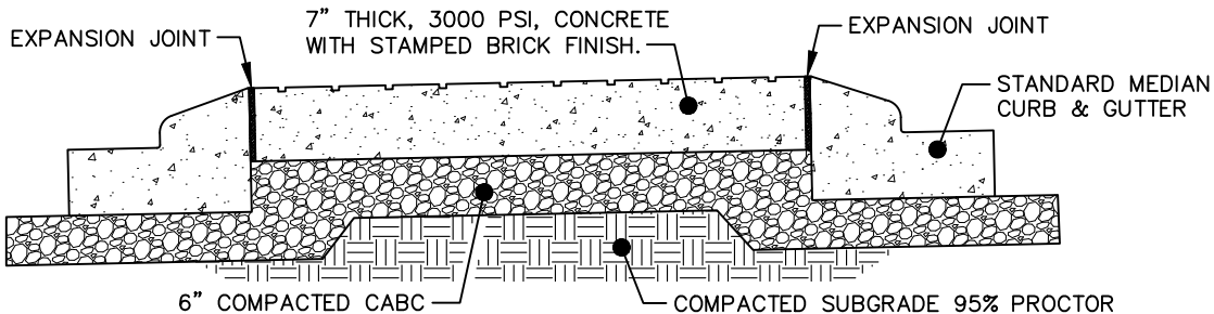
STAMPED CONCRETE MEDIAN SECTION VIEW (USE THIS DETAIL ONLY ON NCDOT MAINTAINED STREETS)
