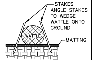
STAKE INSTALLMENT CROSS SECTION
