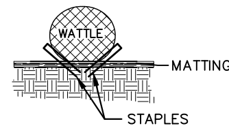
STAPLE INSTALLMENT SECTIONS
