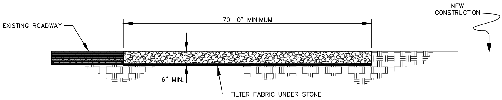
CROSS SECTION
