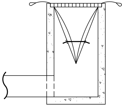
INSTALLATION DETAIL
