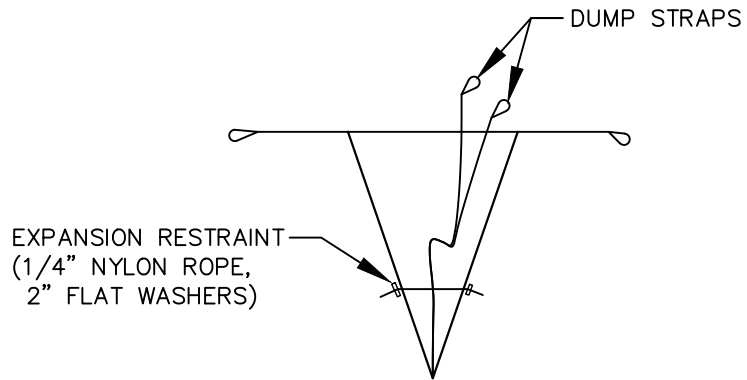
BAG DETAIL
