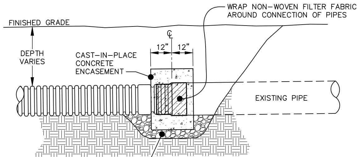
FINISHED CONNECTION SECTION VIEW
