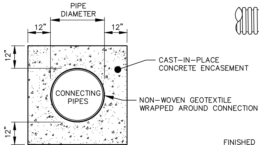
CONCRETE ENCASEMENT CROSS SECTION
