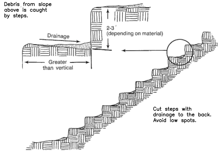
Figure 6.03b Stair stepping cut slopes
