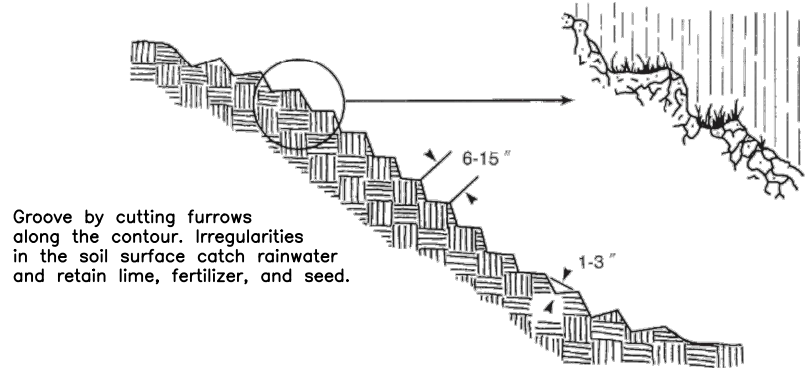
Figure 6.03c Grooving slopes
