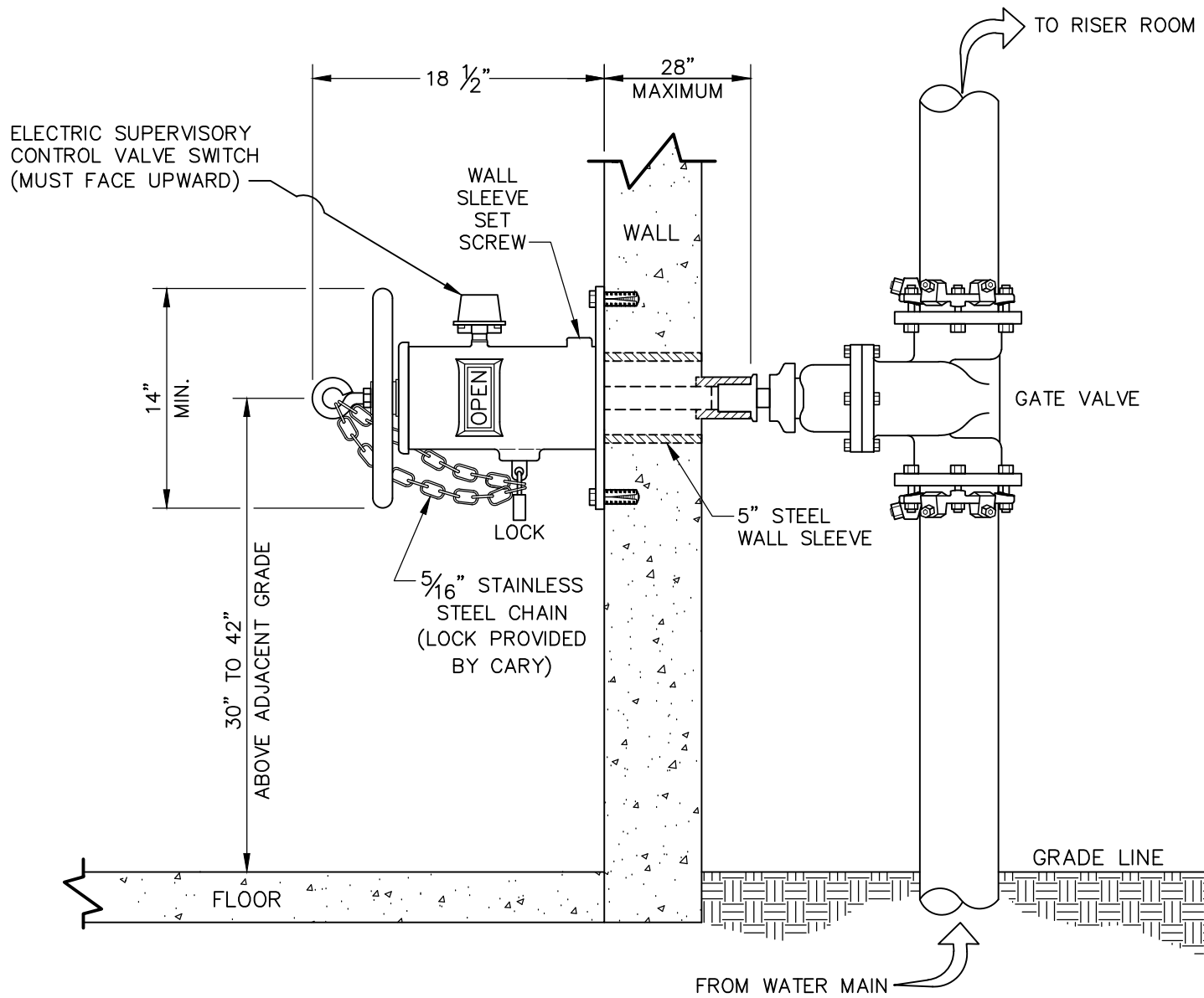
WALL MOUNTED INDICATOR VALVE
