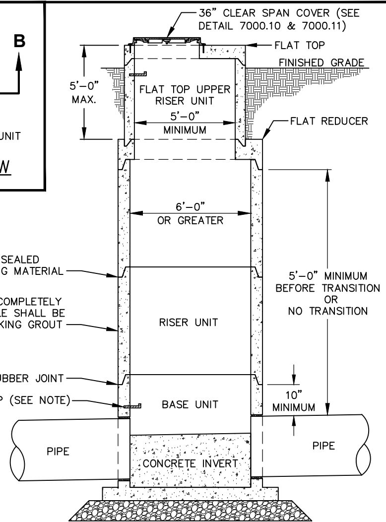
SECTION B-B
