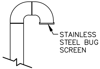
VENT DETAIL
