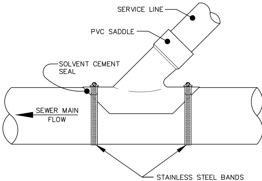
PVC MAIN
