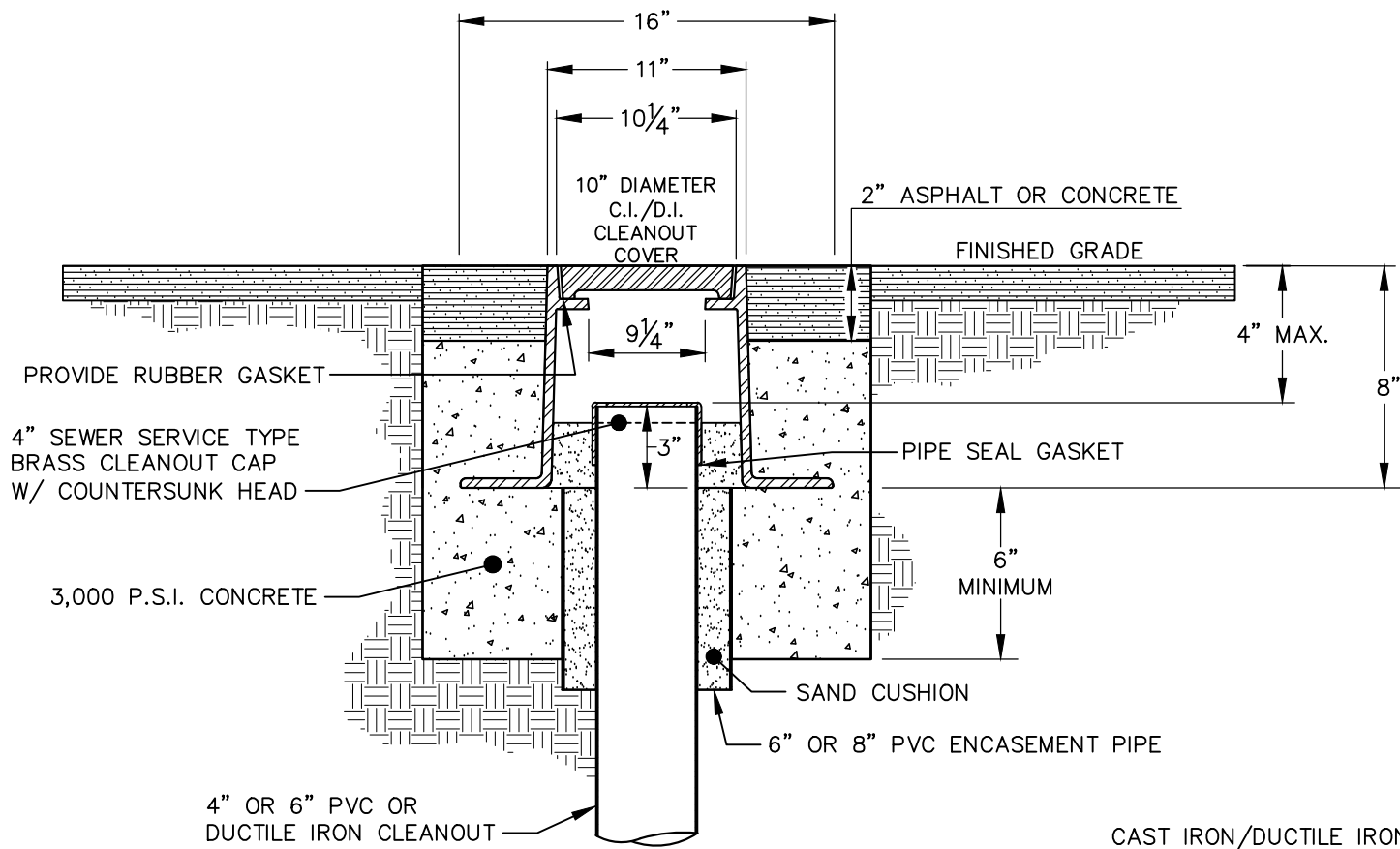
SECTION VIEW
