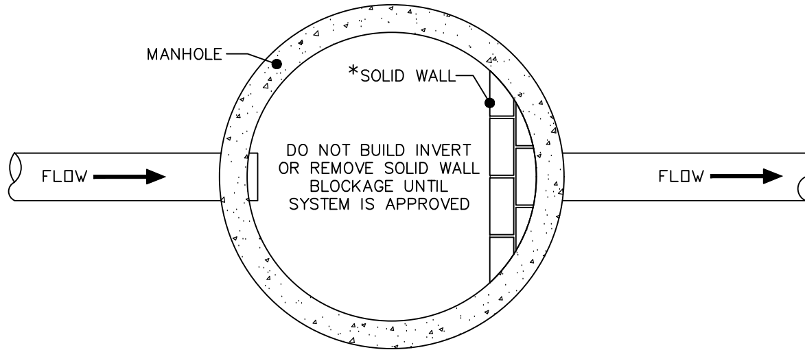
PLAN VIEW
