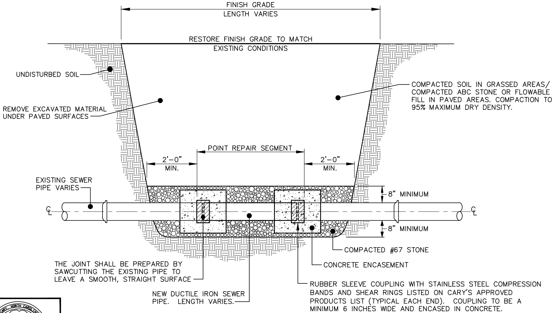
SECTION VIEW
