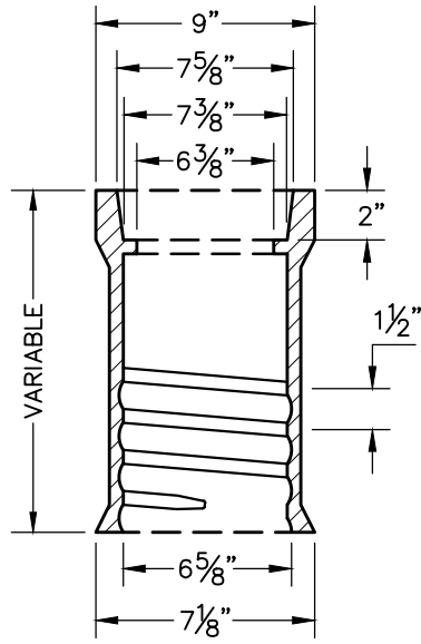
TOP SECTION
