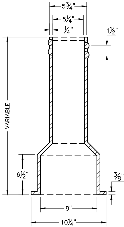
BOTTOM SECTION
