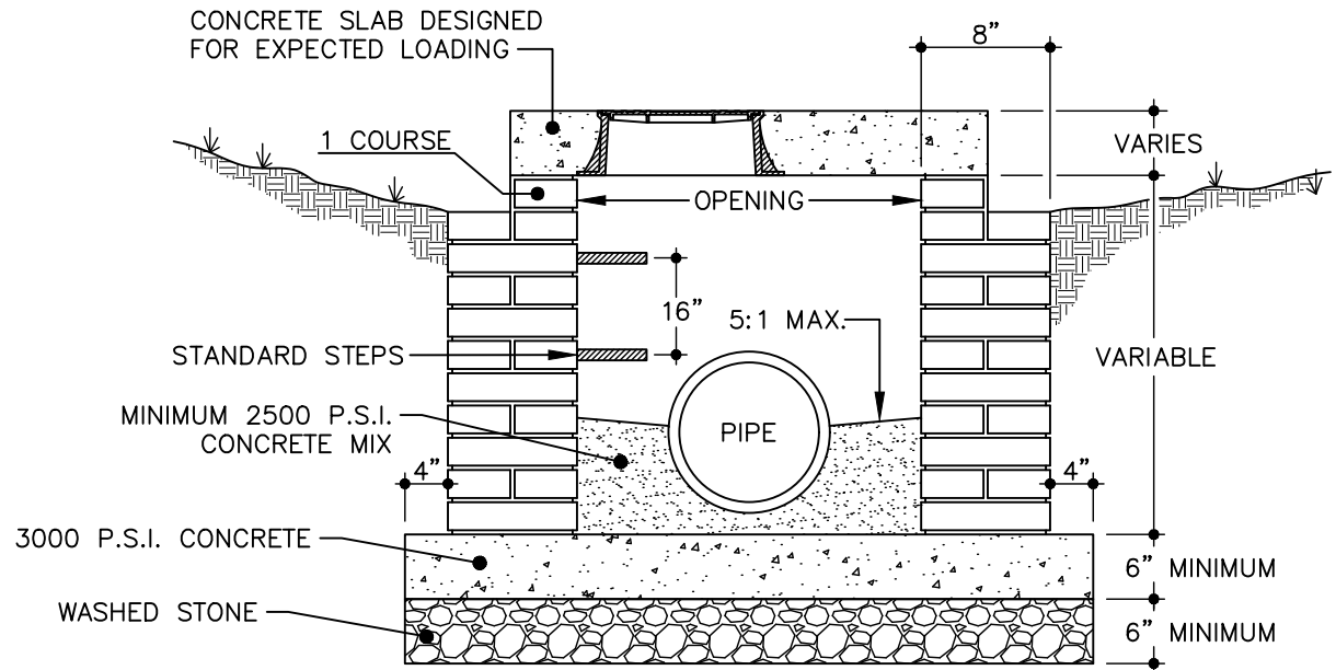
SECTION
