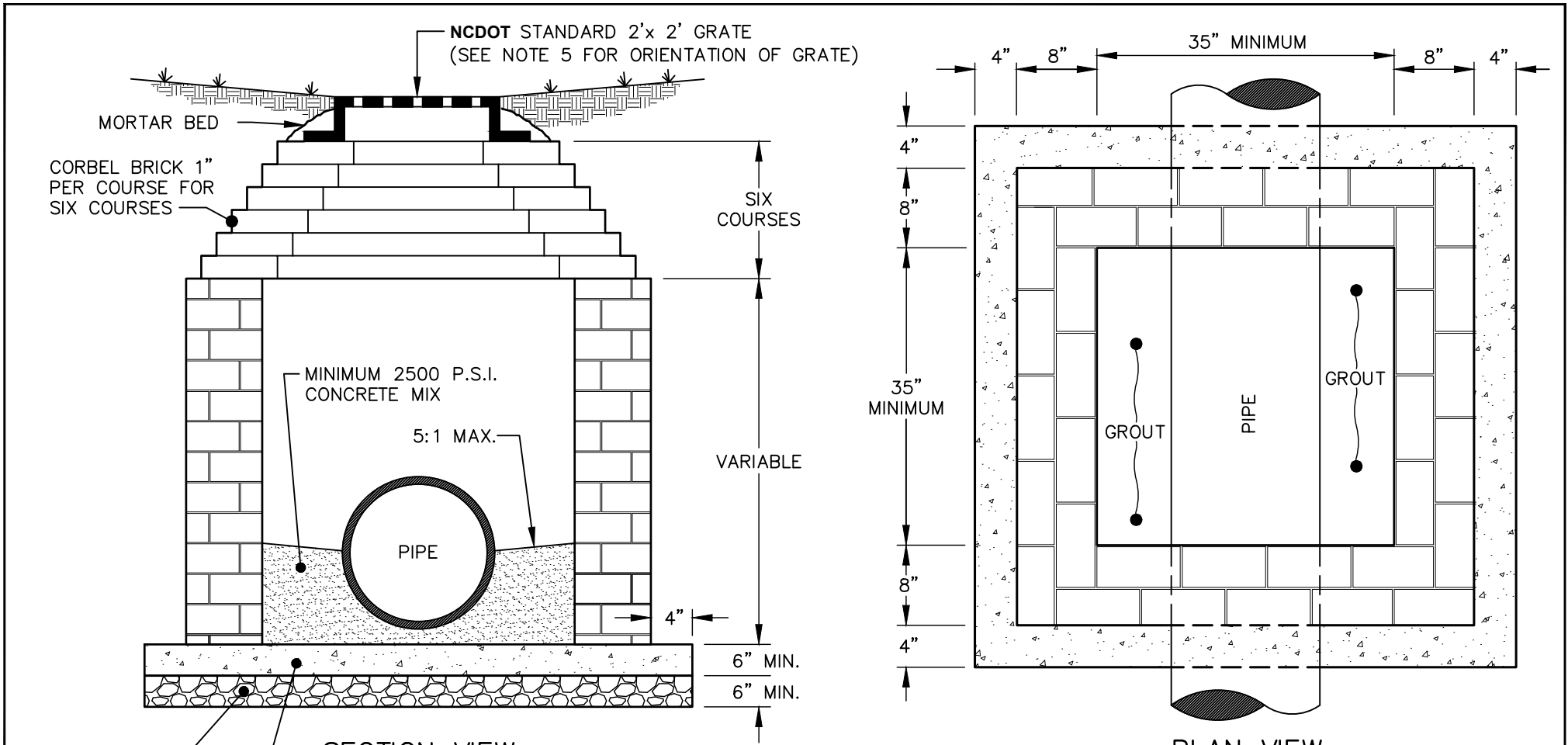
SECTION VIEW
