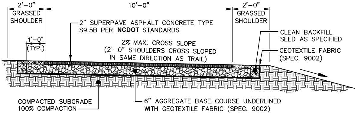
TYPICAL SECTION
