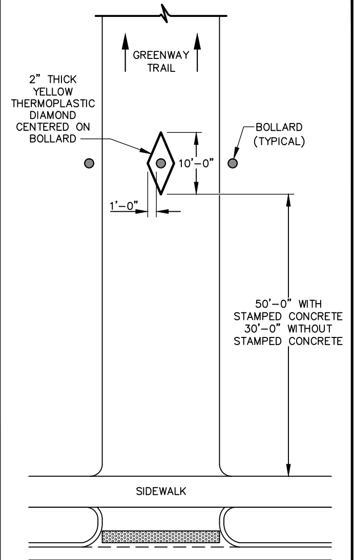
PLAN VIEW
