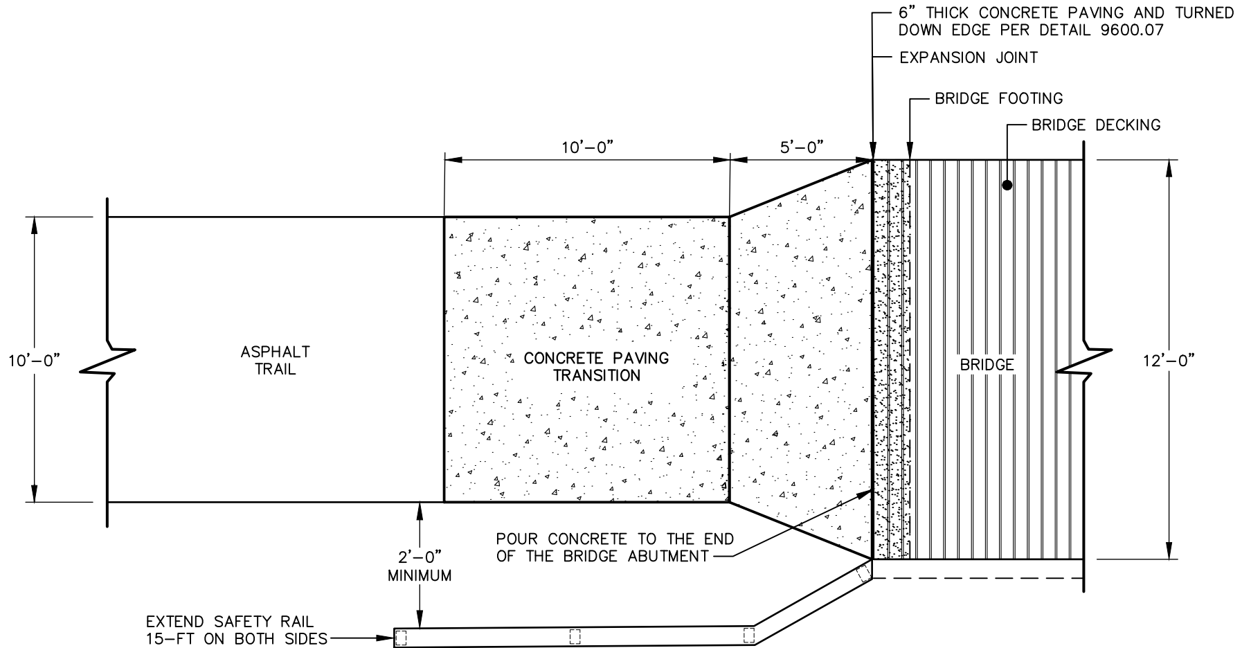
PLAN VIEW
