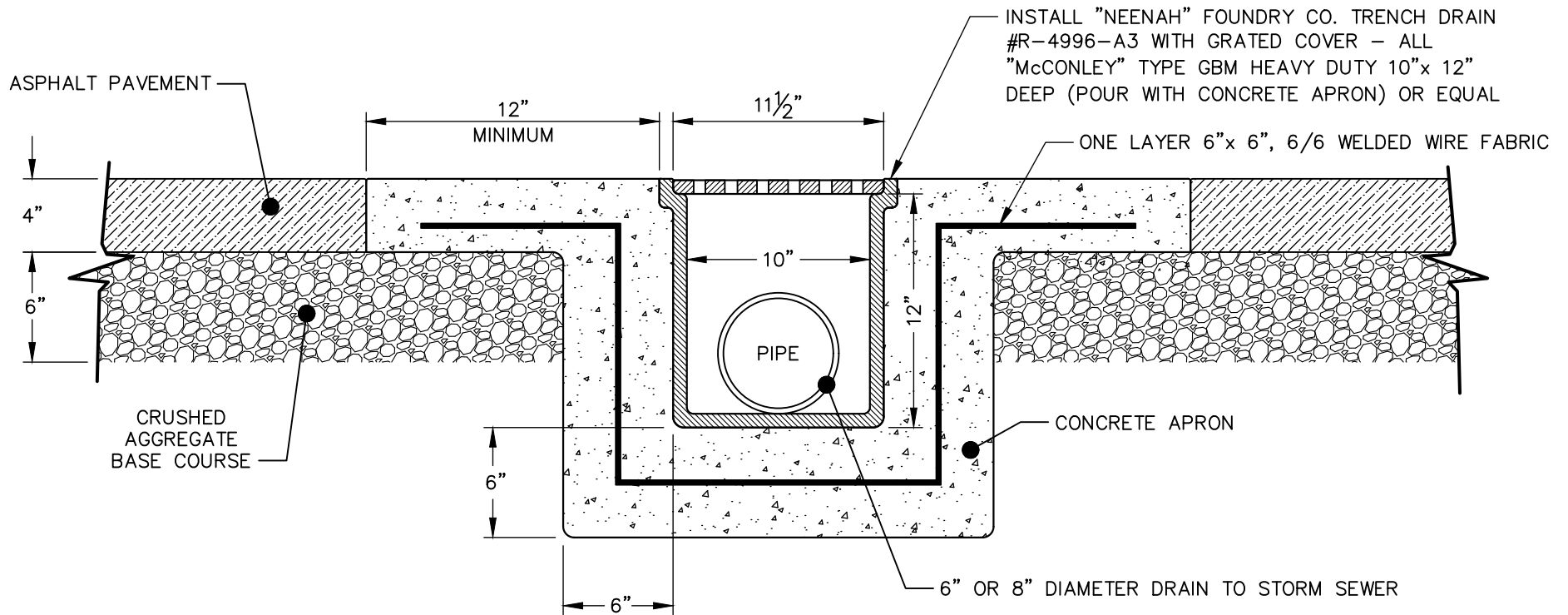
SECTION VIEW
