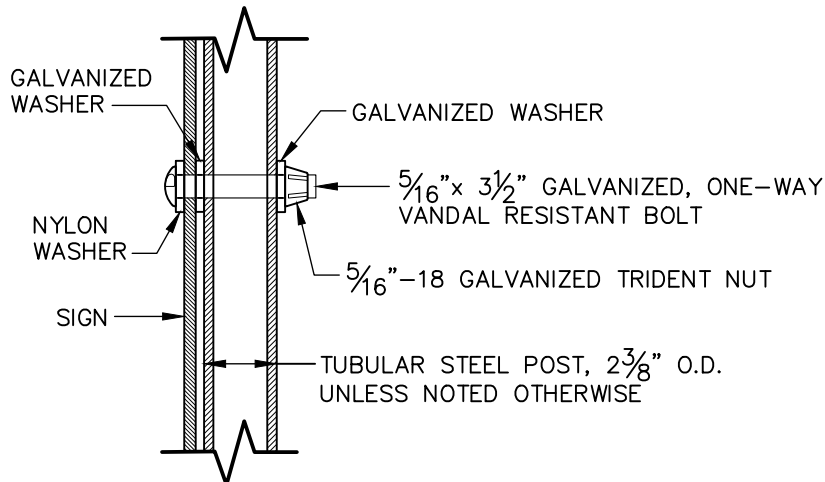
POST MOUNTING DETAIL
