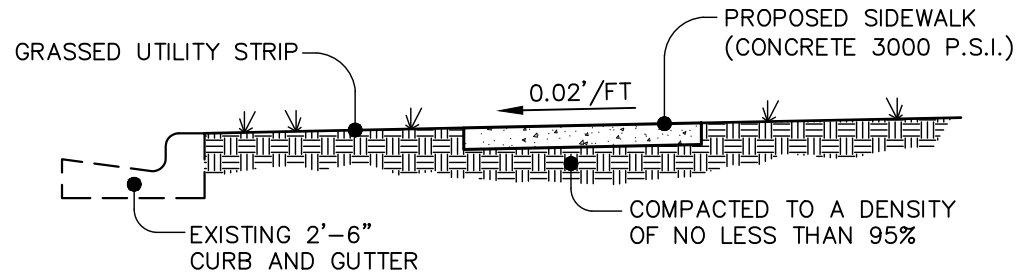
TYPICAL SECTION
