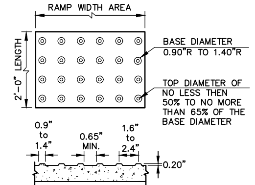
DETECTABLE WARNING DOMES
