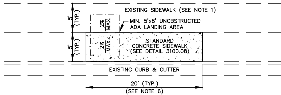
LANDING PAD WITH SIDEWALK AND UTILITY STRIP
