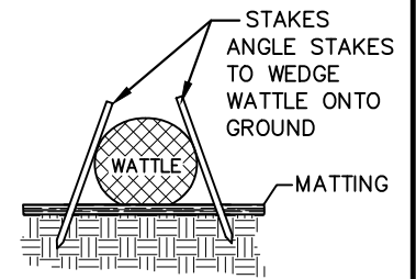
STAKE INSTALLMENT CROSS SECTION
