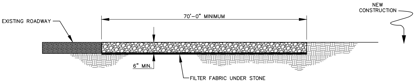
CROSS SECTION
