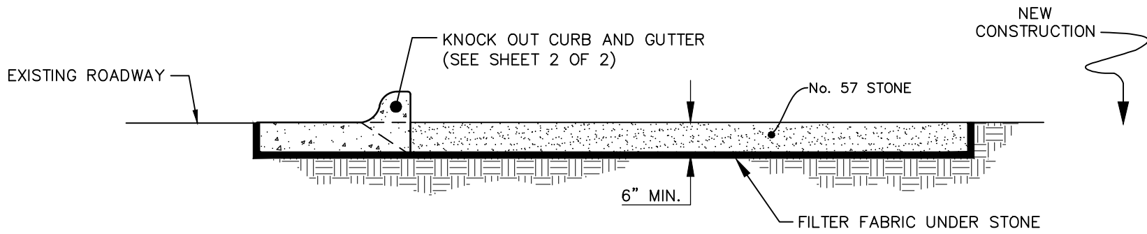
CROSS SECTION
