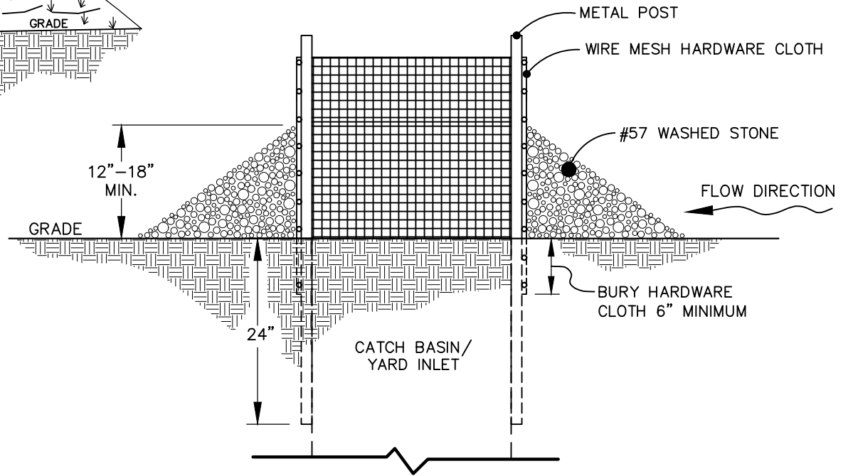
FRONT SECTION VIEW
