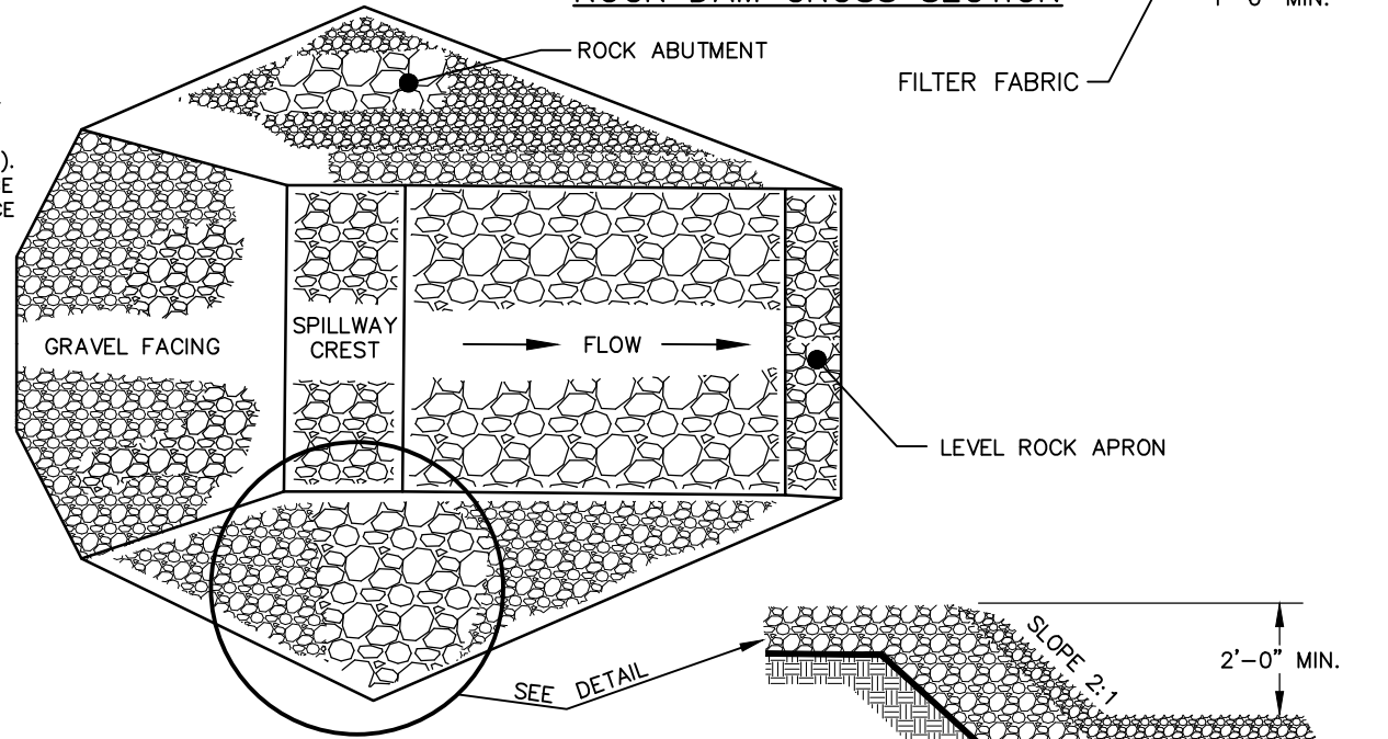
PLAN WITH SPILLWAY DETAIL
