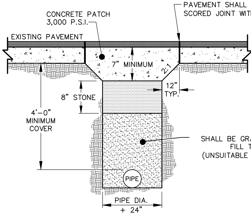
CONCRETE PAVEMENT
