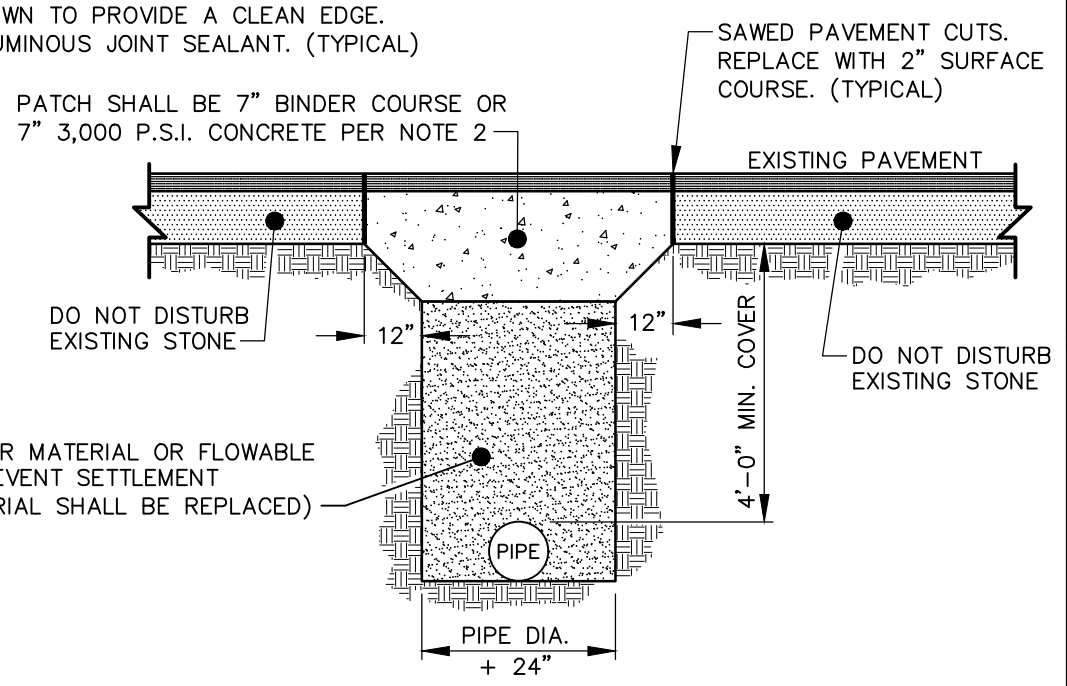
ASPHALT PAVEMENT
