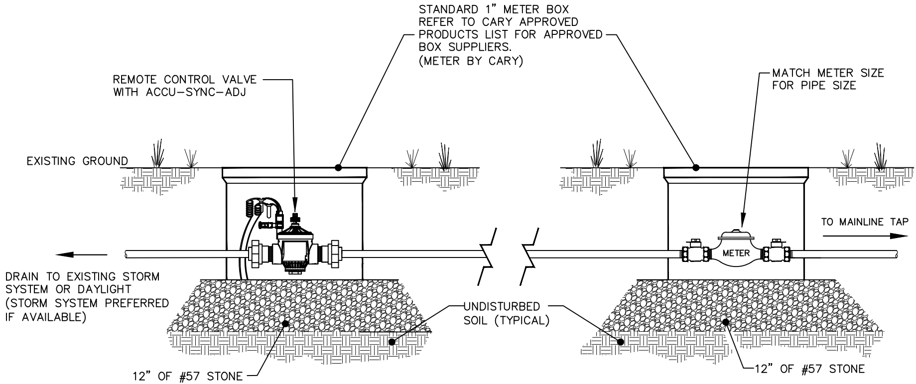
SECTION VIEW
