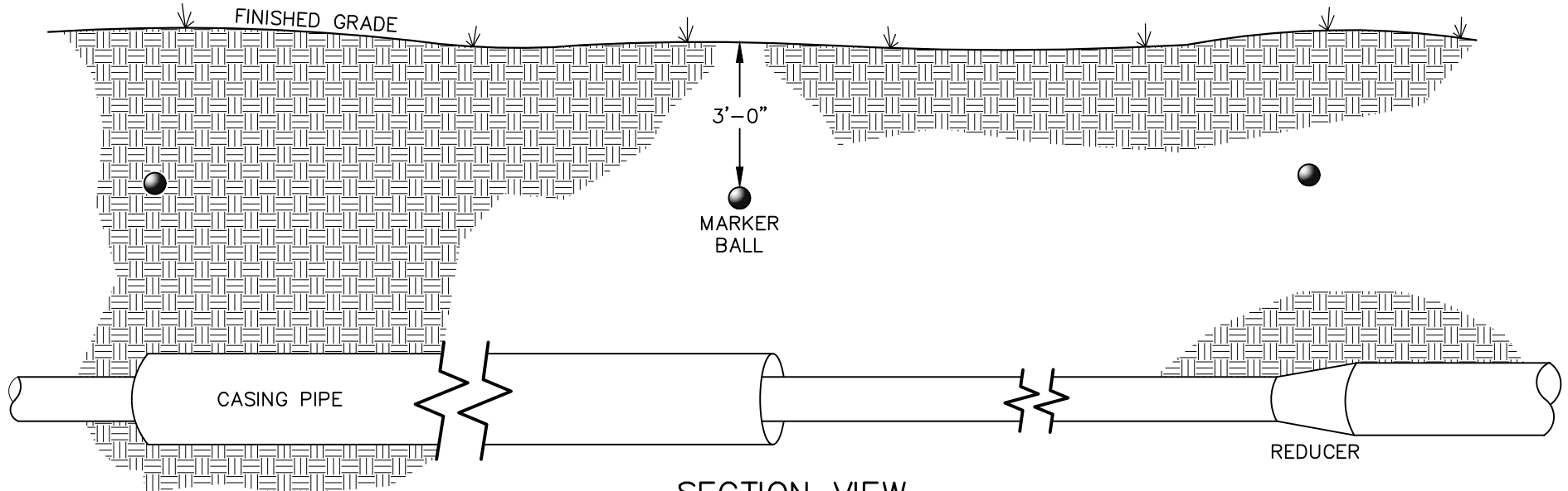
SECTION VIEW
