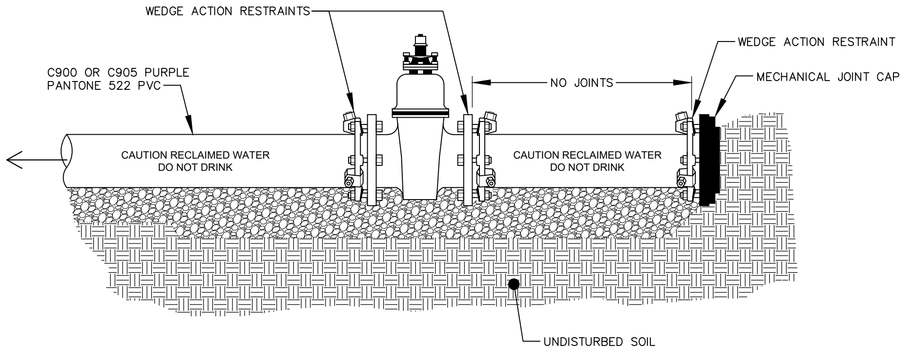
SECTION VIEW
