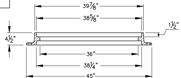
FRAME SECTION
