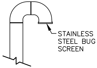
VENT DETAIL
