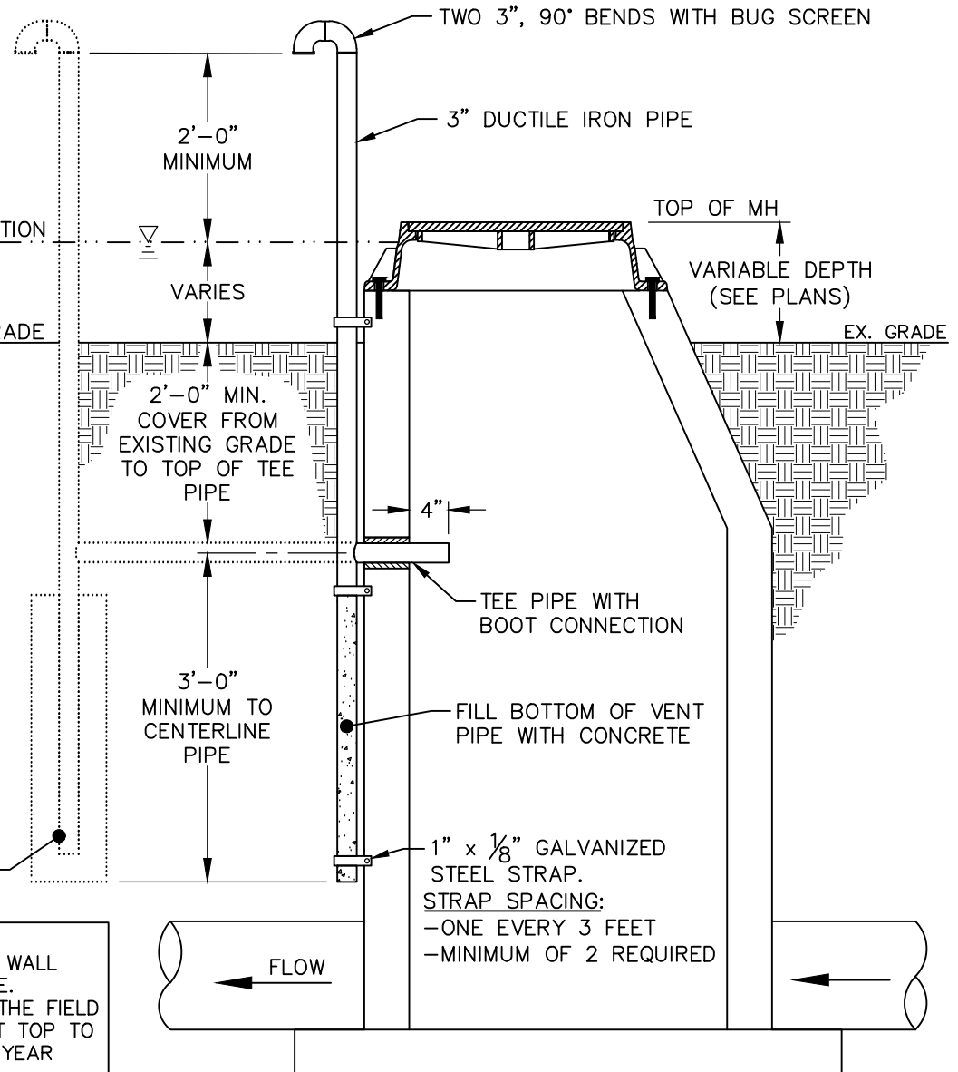
SECTION VIEW
