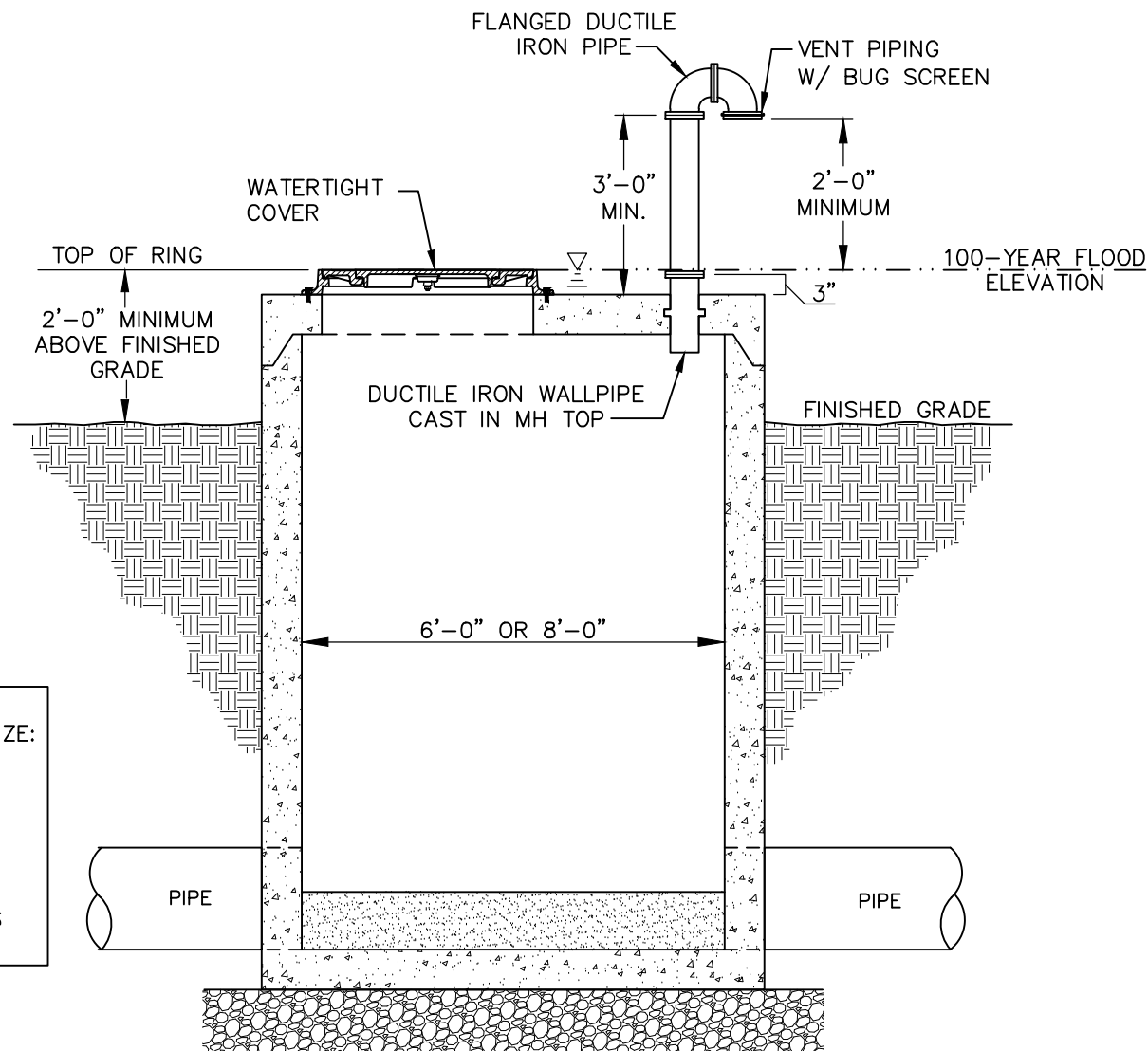
SECTION VIEW
