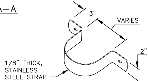
STRAP DETAIL
