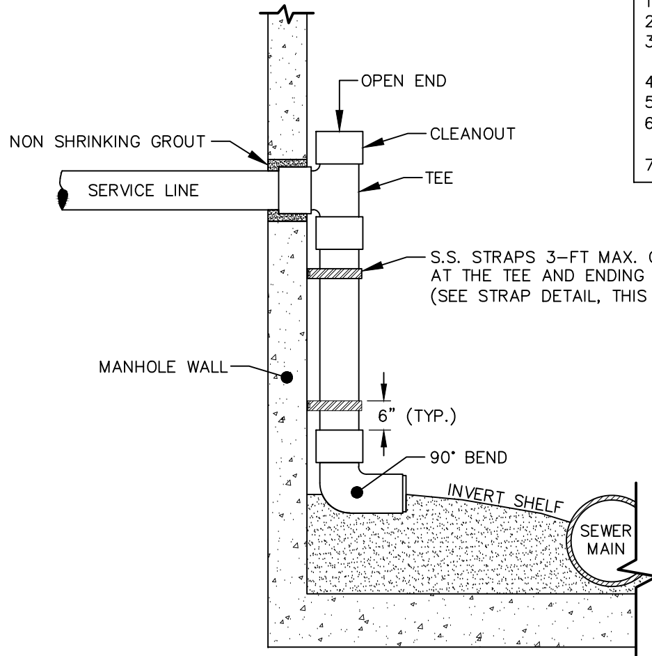
SECTION VIEW
