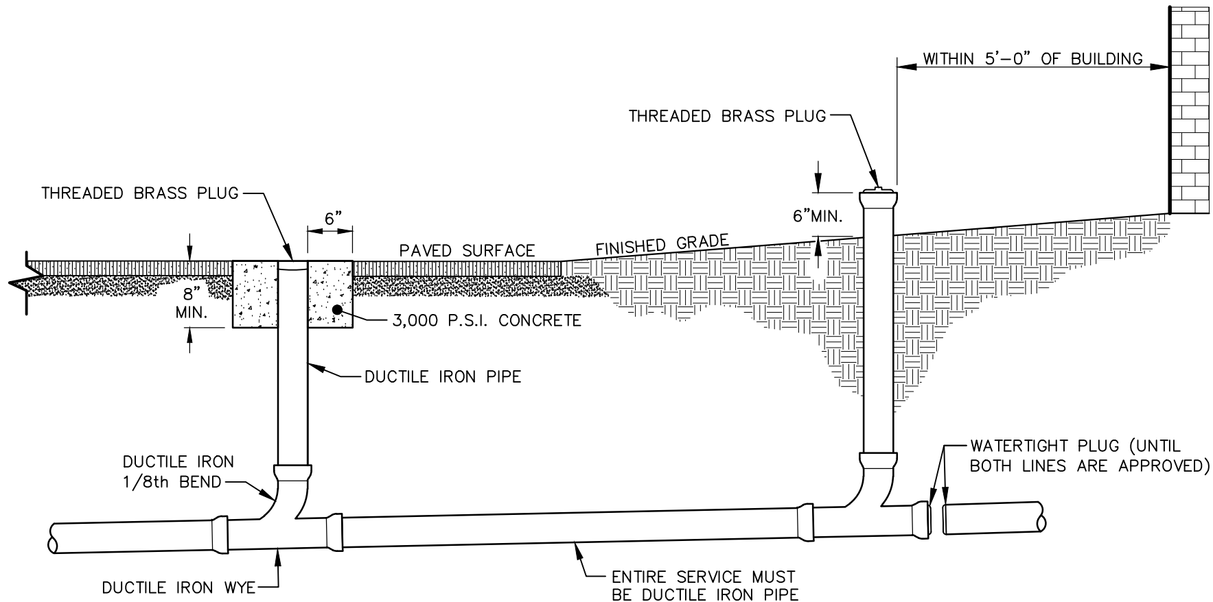
SECTION VIEW
