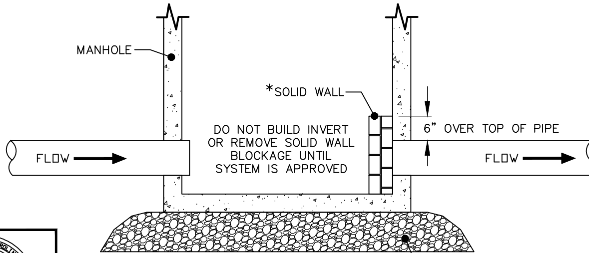
SECTION VIEW
