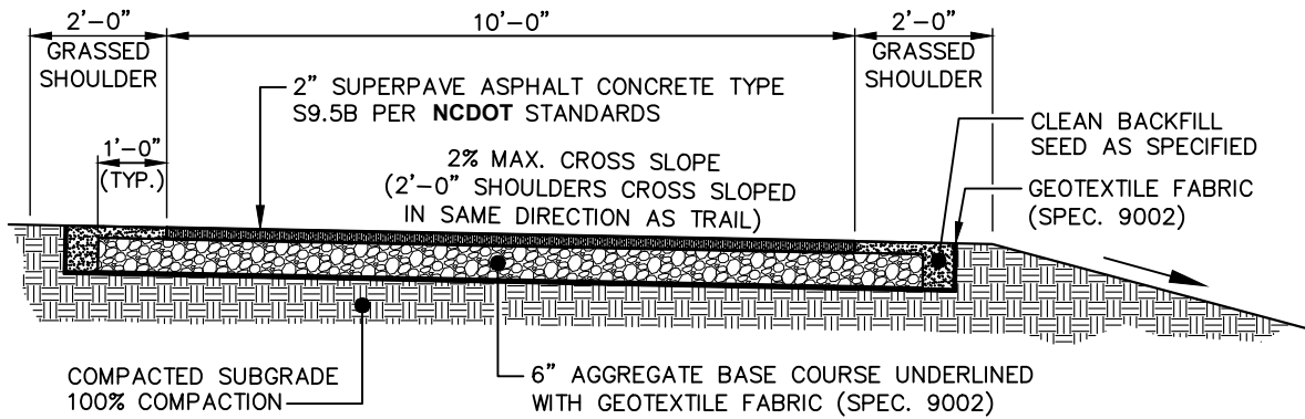
TYPICAL SECTION
