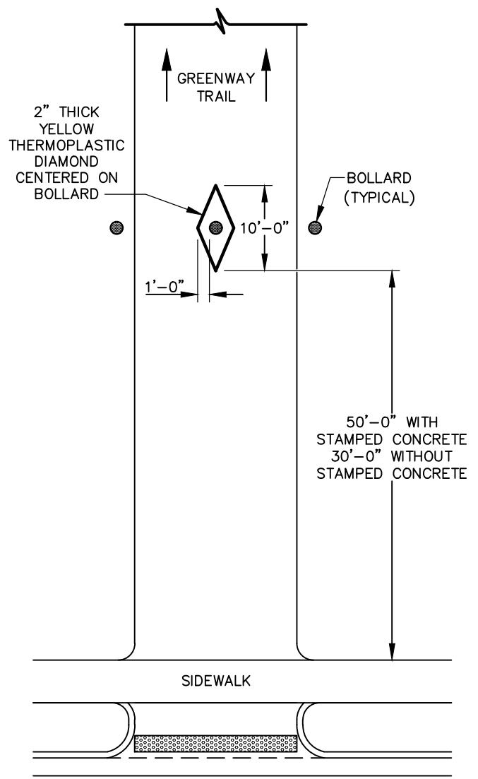
PLAN VIEW
