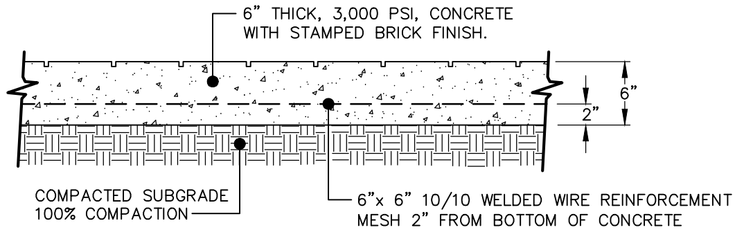
SECTION VIEW
