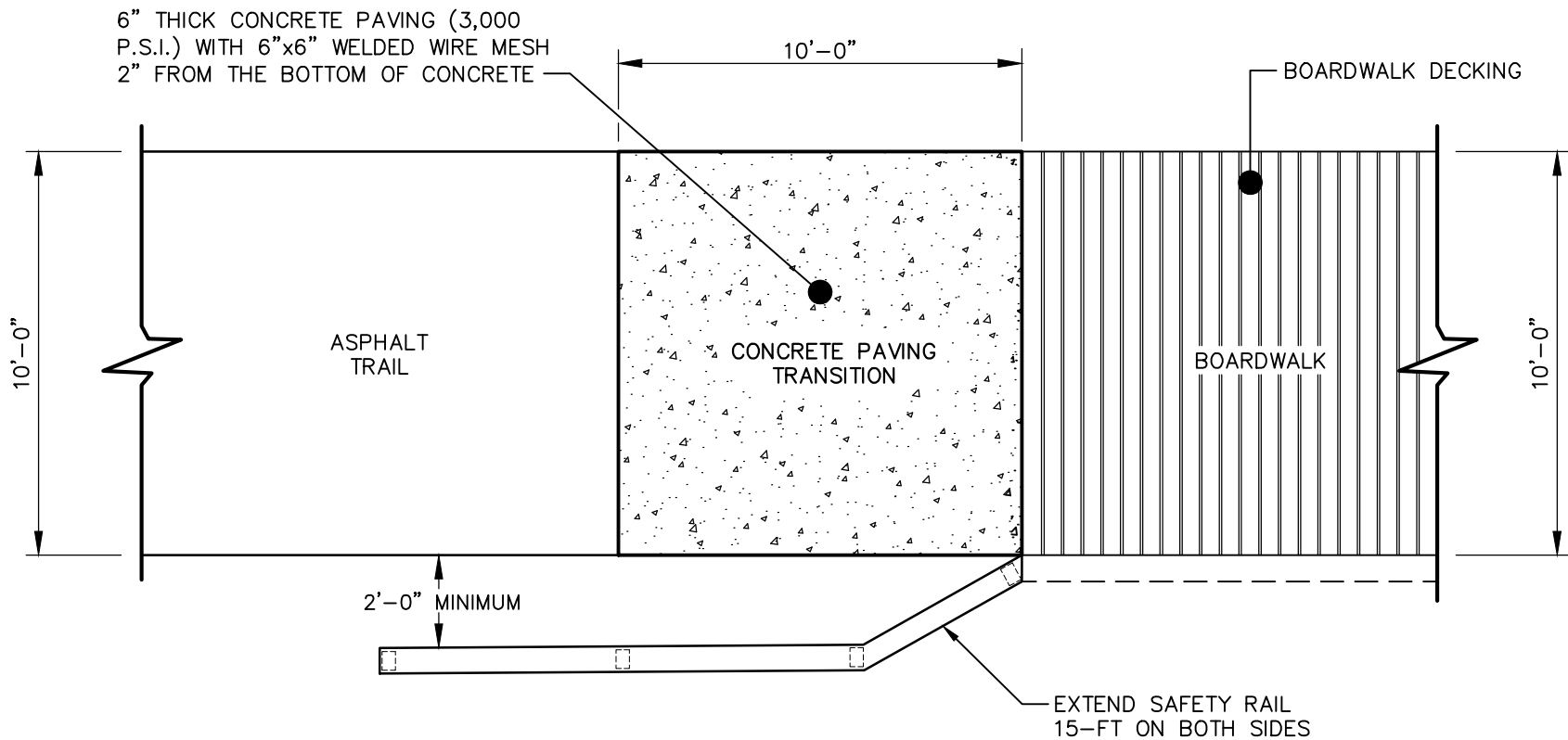
PLAN VIEW
