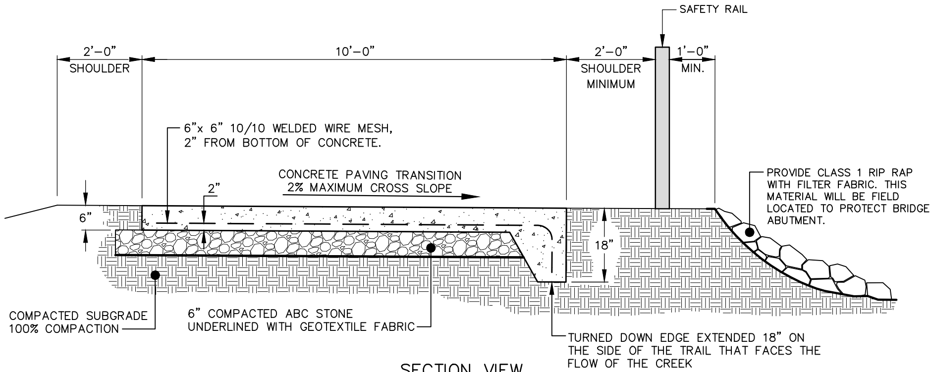
SECTION VIEW
