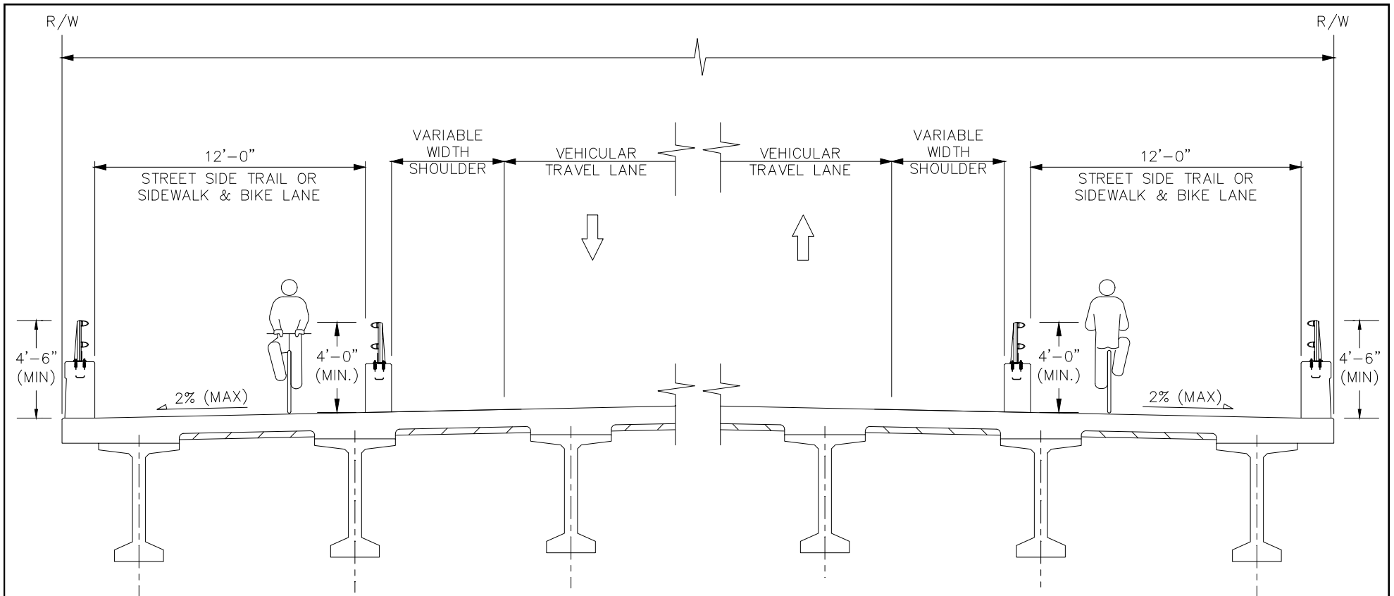
TYPICAL SECTION
