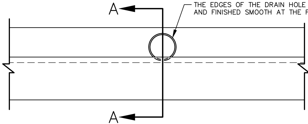
FRONT VIEW
